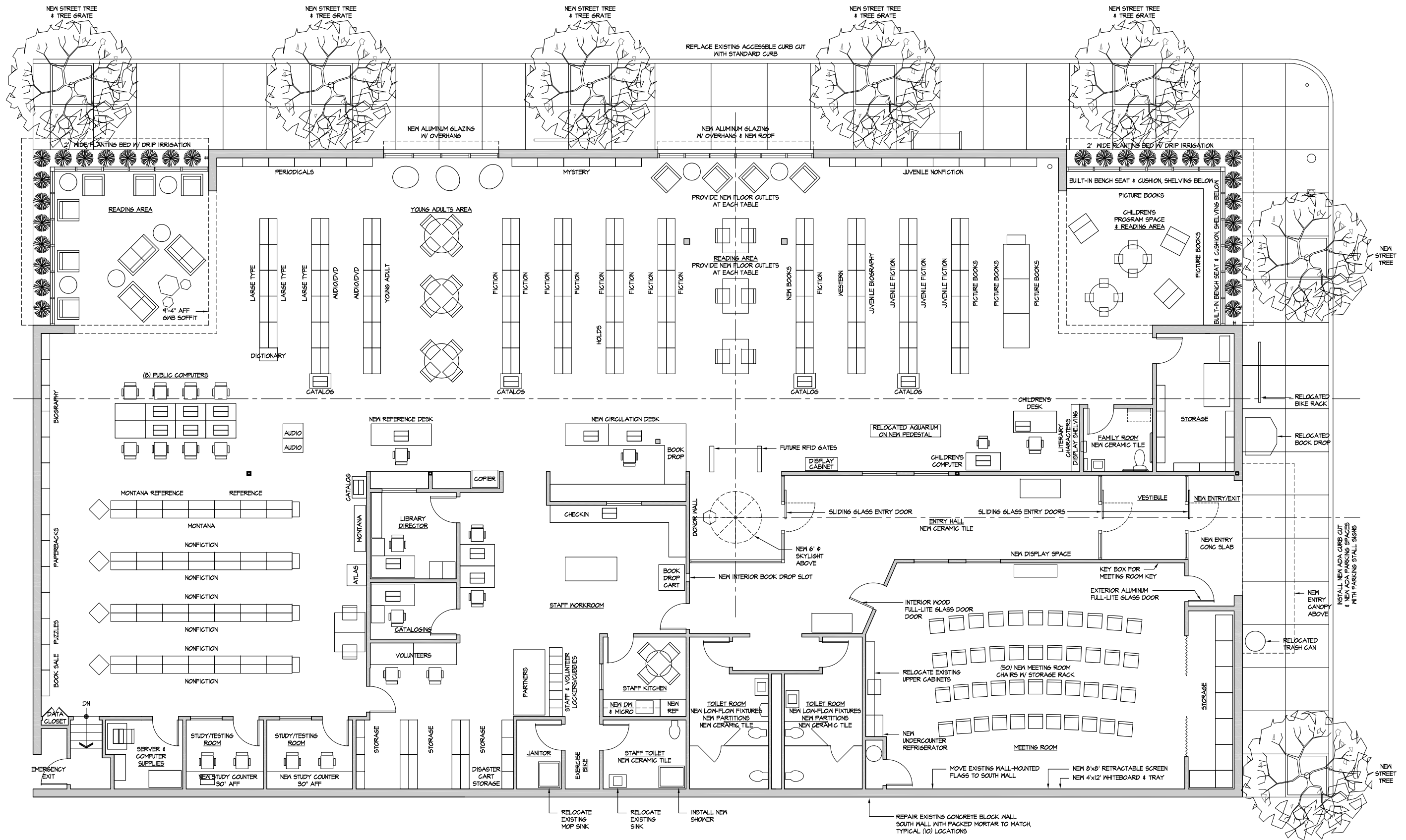
PROPOSED BUILDING & SITE PLAN scale: 1/4" = 1'-0"
